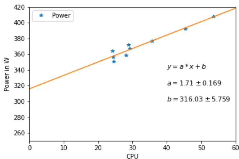
Figure 3: Determining P_{idle} from the measured data points
