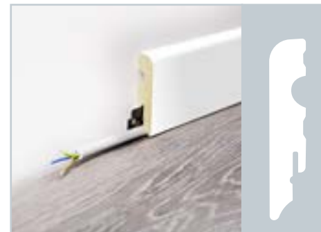
Skirting board 15/70 MDF base 15 × 70 × 2400 mm
