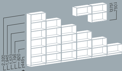
Filing shelves *
