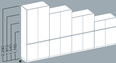
Combination cabinets
