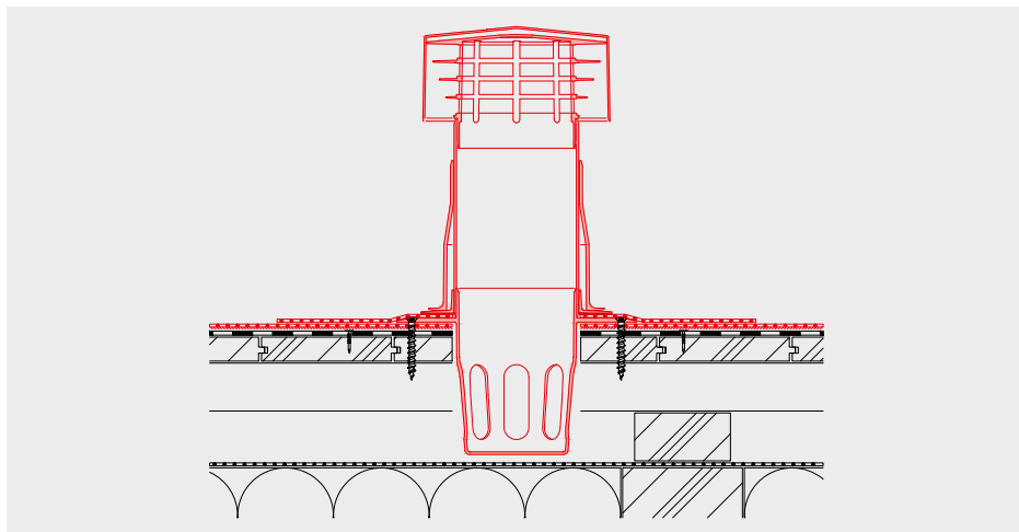
alwitra-Kaltdachlüfter
