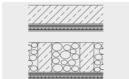
Betonplatten/Rasengitterstein
