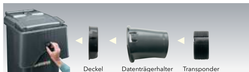
Transponder Montage
